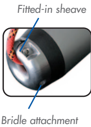
Bridle attachment
